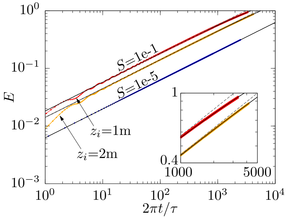
Figure 8. Temporal evolution of the dilution index. Blue dots represent numerical results for S=1e-5 , red and orange dots for S=1e-1 with z_i=1m and z_i=2m respectively, black solid lines represent predictions from the equation (49) and gray dashed lines represent results for the linear regime ( E(t) \propto t^{1/2} ). The inset magnifies the subdiffusive regime of the dilution index as E(t) \propto t^{1/4} .
