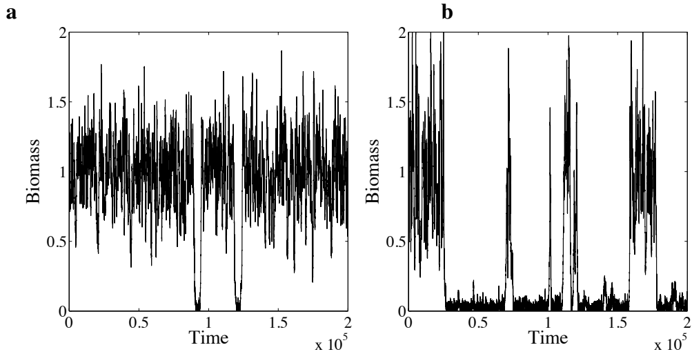
FIG. 6: Long-time biomass time series for the systems of Figure 4. The shift from the vegetated to the non-vegetated state leads to larger system fluctuations and intermittent behavior. The model parameters are the same as in Figure 4. In these two scenarios, the mean annual precipitation is the same, but the mean lag time between storms and mean precipitation depths are different: \alpha = 0.012 , \lambda = 1/3 (case a ), and \alpha = 0.032 , \lambda = 1/8 (case b ).
