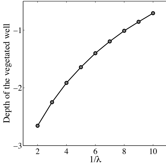
FIG. 8: Depths of the vegetated well for \alpha \times \lambda = 0.004 as a function of the mean inter-storm waiting time 1/\lambda . The model parameters are the same as in Figure 4. The depth of the well can be interpreted as the attracting strength of the vegetated state, and is a measure of its resilience against random perturbations. In the case of shallow wells, which are characteristic of the larger events separated by larger intervening periods (large \lambda , Fig. 7b) the system can easily fall into the basin of attraction of the non-vegetated state. These systems are also characterized by higher variability and intermittency (Fig. 6b).
