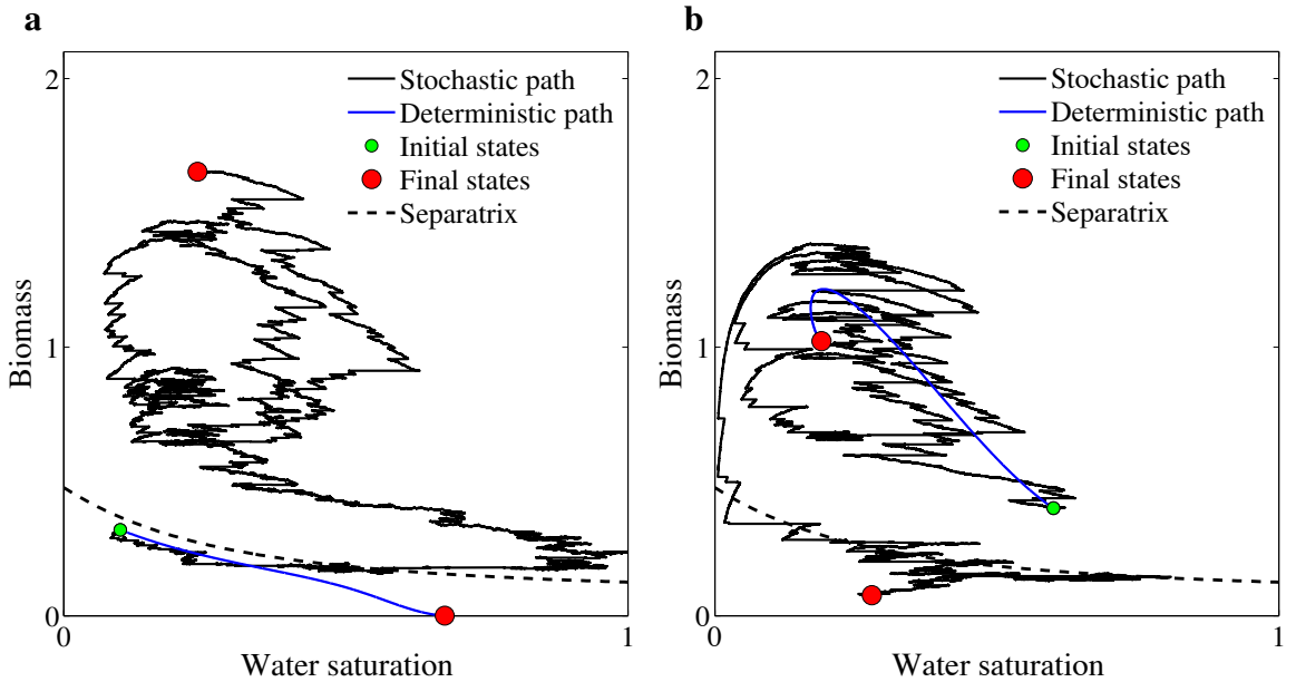
FIG. 3: (Color online) Stochastic ecosystem trajectories for (a) frequent rain events with low amplitude, and (b) rare storm events with large amplitude. The model parameters are the same as in Figure 1 with E = 0.004 and a mean daily precipitation of I = 0.004 . The mean daily precipitation is the same for both cases, but the mean lag time between storms and mean precipitation depths are different: \alpha = 0.016 , \lambda = 1/4 (a), and \alpha = 0.04 , \lambda = 1/10 (b).
