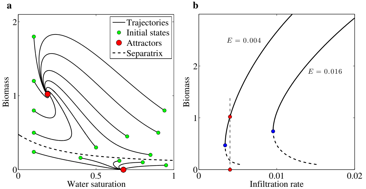
FIG. 1: (Color online) Behavior of the deterministic system (1a-1b). The dynamical system is deterministic when the infiltration rate is constant, and the gaussian noise terms are neglected. For parameter values that are typical of arid and semiarid environments, the system exhibits two alternative stable states. a , Sample trajectories for E = 0.004 , I = 0.004 . Furthermore, we set \beta = 0.004 , \gamma = 0.02 , \delta = 0.004 , \mu = 0.008 , k = 0.2 , b_0 = 0.4 , and K_s = 0.002 . The system is bistable, and we may arrive at either of the attractors depending on the initial condition. The region of initial values in phase space that converges to a given attractor is called the basin of attraction of that stable point. b , Bifurcation diagrams using the recharge rate, I , as the bifurcation parameter. The two curves represent the biomass at equilibrium that corresponds to two evaporation rates, E = 0.004 and E = 0.016 . For small infiltration rates, the system has two alternative stable states: a vegetated and a non-vegetated state (red dots).
