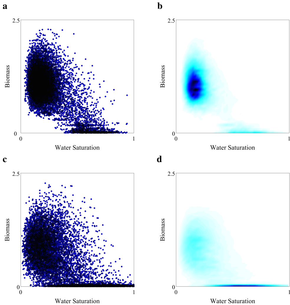
FIG. 5: (Color online) Empirical joint probability density functions from Monte-Carlo simulation of the model equations (5a-5b) for the same scenarios as in Figure 4. (b, d) Steady-state joint probability density functions of soil moisture and biomass as in Figure 4. (a,c) Scatter plot of system states during the time evolution of soil moisture and biomass. Right panels, normalized histograms of system states.
