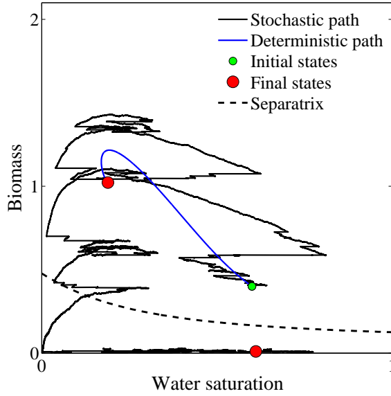
FIG. 2: (Color online) Stochastic ecosystem trajectory for a power-law interstorm waiting time with exponent a = 0.6 and characteristic time scale \tau_c = 10 and average recharge depth \alpha = 0.04 such that \alpha/\tau_c = 0.004 is equal to the recharge rate for the deterministic model illustrated in Figure 1. The remaining model parameters are the same as in Figure 1 with E = 0.004 . The trajectory starts in the vegetated basin and ends asymptotically in the non-vegetated basin.
