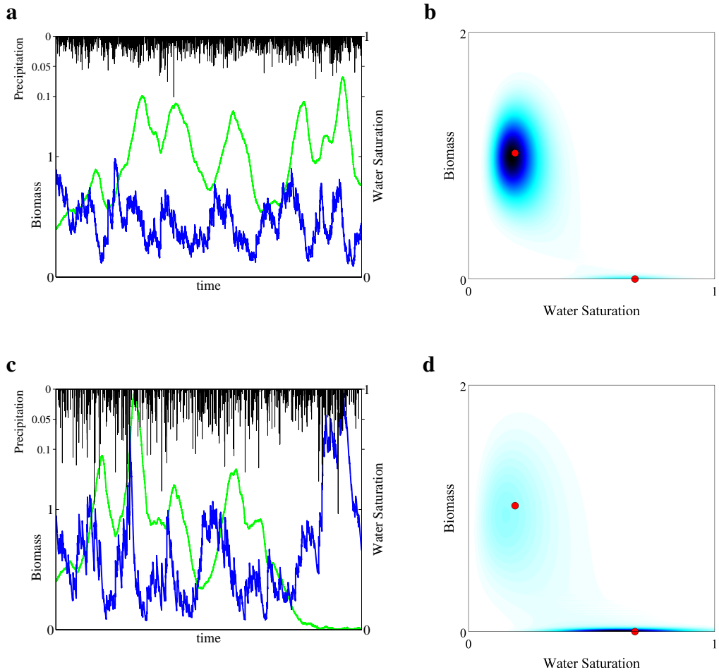
FIG. 4: (Color online) a, c , Sample realizations of the model equations (5a-5b), coupling rainfall, soil moisture and vegetation biomass with stochastic rainfall and gaussian perturbations. The model parameters are the same as in Figure 1 with E = 0.004 and the mean daily precipitation I = 0.004 . In these two scenarios, the mean annual precipitation is the same, but the mean lag time between storms and mean precipitation depths are different: \alpha = 0.012 , \lambda = 1/3 (cases a–b), and \alpha = 0.032 , \lambda = 1/8 (cases c–d). (b, d) Steady-state joint probability density functions of soil moisture and biomass, calculated with our stochastic model, Eq. (27). In the case of frequent, small storm events, the PDF has a clear maximum around the vegetated stable state (b). In contrast, for infrequent, larger precipitation events, the probability of the non-vegetated system states increases (d). The cumulative probability to be in the vegetated basin is 0.92 for scenario 1 (b) and 0.6 in scenario 2 (d).
